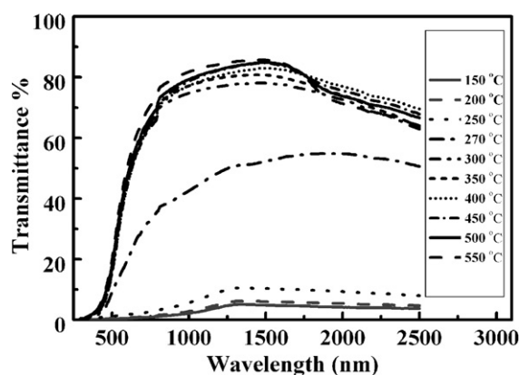
Fig. 8. Typical data of spectral normal transmittance of (\text{CdO})_{0.9}(\text{In}_2\text{O}_3)_{0.1} films annealed at different temperatures for 15 min.
