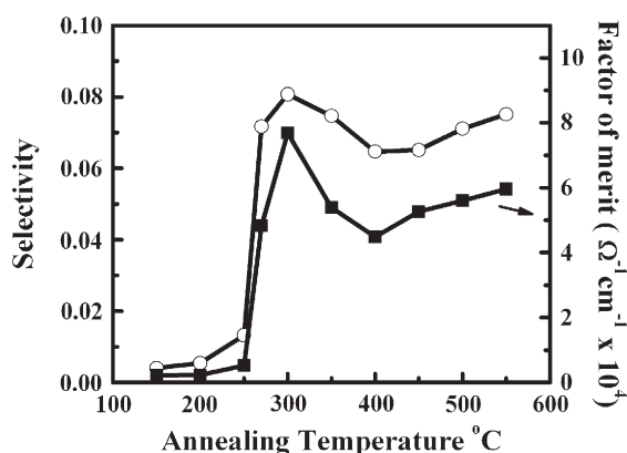
Fig. 9. Annealing temperature dependence of the factor of merit and selectivity for (\text{CdO})_{0.9}(\text{In}_2\text{O}_3)_{0.1} films.
